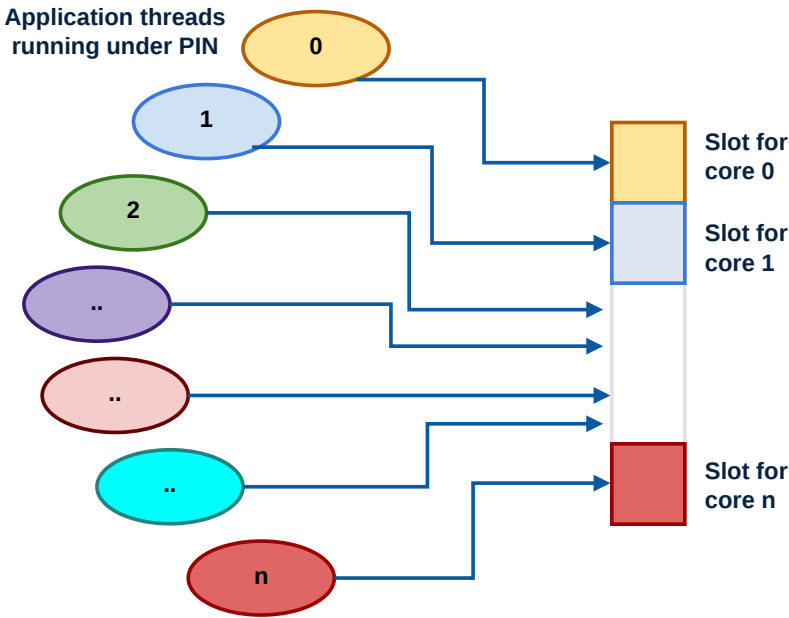
Fig. 3. Structure of the shared memory segment
