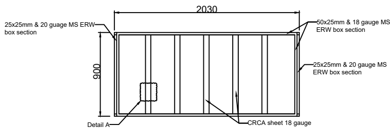
Cot frame detail
